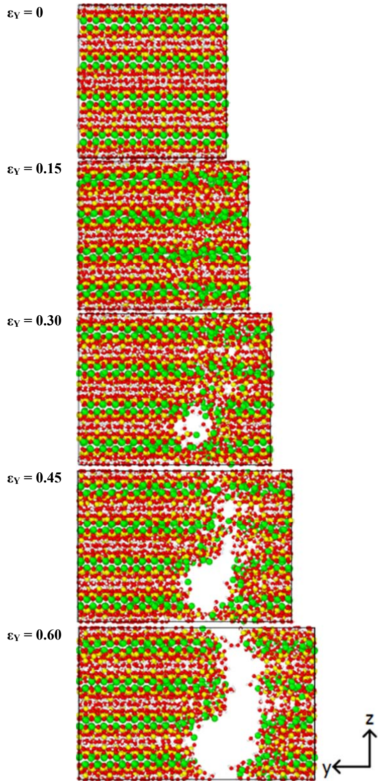
Figure 5-6 Progress of damage to the molecular structure of tobermorite 11 Å, under tensile strains in the y direction. (Green: Ca; Yellow: Si; Red: O; White: H)
