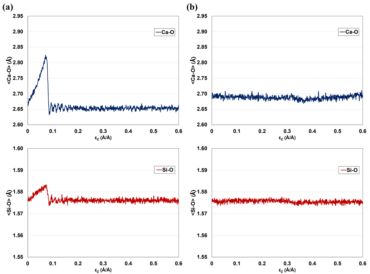
Figure 5-8 Average bond length as a function of strain along the z_z direction of (a) tobermorite 11 Å and (b) tobermorite 14 Å.
