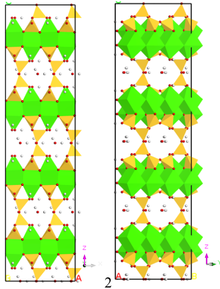
Figure 2-2 Two views of the 2a \times 2b \times 2c supercell of tobermorite 11 Å (Green: Ca; Orange: Si; Red: O; and White: H)
