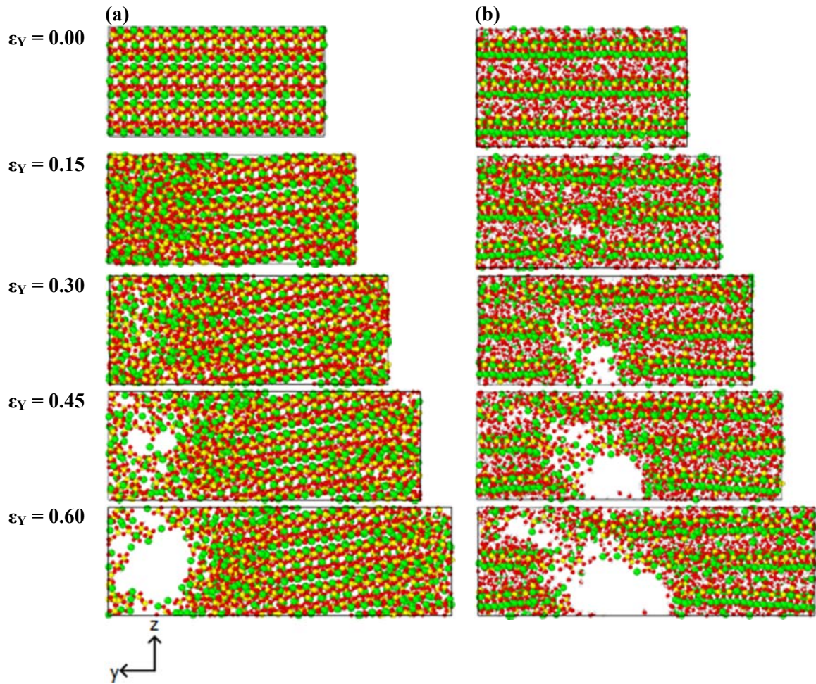
Figure 5-20 Process of damage to the molecular structure of (a) tobermorite 9 Å and (b) jennite under tensile strains in the y direction. (Green: Ca; Yellow: Si; Red: O; White: H)
