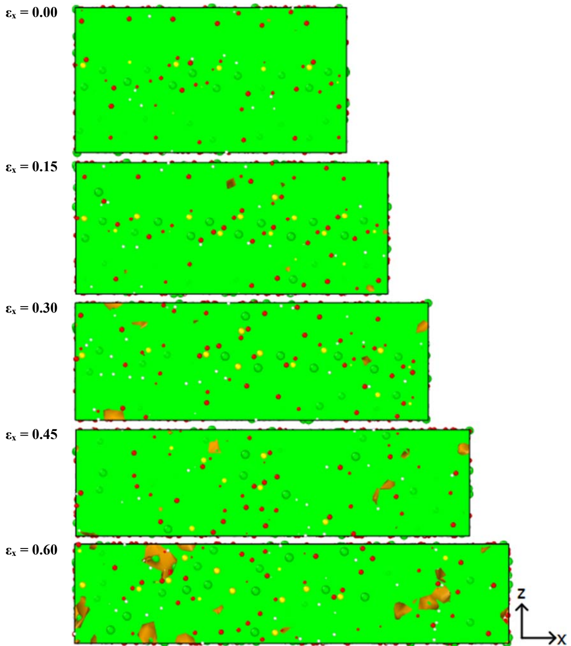
Figure 5-17 The formation and distribution of local voids in the structure of jennite subjected to the uniaxial tensile strain in the x direction.
